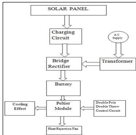
Fig 3: Block Diagram of the Solar AC
